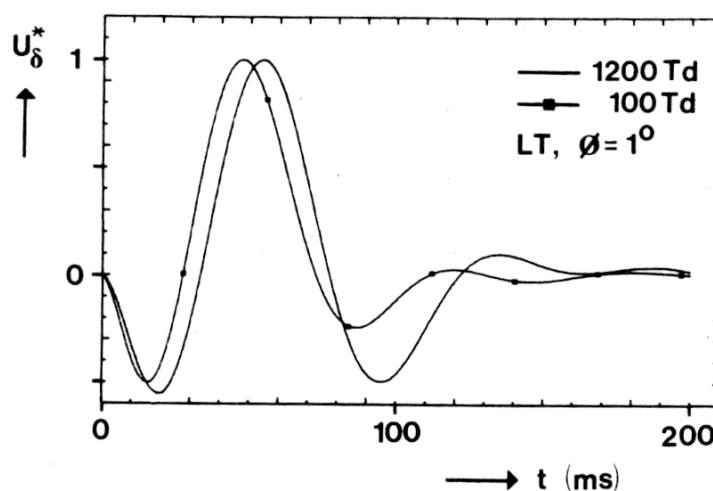
Figure 16. Impulse response functions for two background adaptation levels, estimated using Roufs and Blommaert's signal perturbation technique. Adapted from den Brinker (1989).
