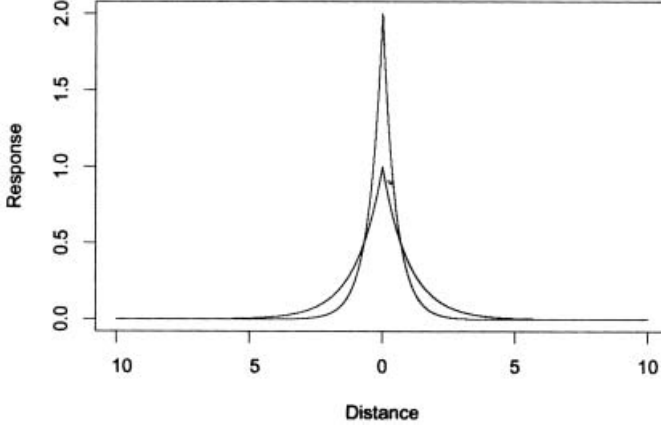
Figure 2. Two receptive fields are shown. A maximal response is elicited from both receptive fields when a stimulus falls in the centre of each receptive field (a 1.0 response for the broadly tuned receptive field; a 2.0 response for the tightly tuned field). Compared to the broadly tuned field, the tightly tuned field's response is stronger for stimuli falling close to the centre and is weaker for stimuli farther from the centre. The crossover point occurs at a distance from centre of 0.7 (approximately).
