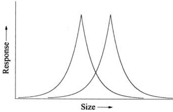
Figure 1. Two receptive fields are shown. These receptive fields are for the same dimension (i.e. size) and accordingly have the same tuning, but are centred at different positions along the dimension. The cluster containing the receptive field on the right prefers larger stimuli than the cluster containing the receptive field on the left.
